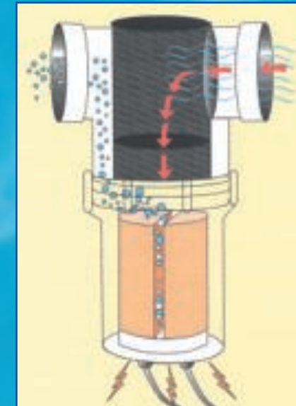
Clearwater's ionization process
